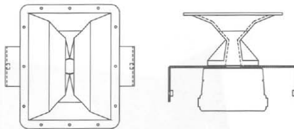
FIGURE 2 - Mounting the HMK-4's U-Bracket Between the Driver and Horn
